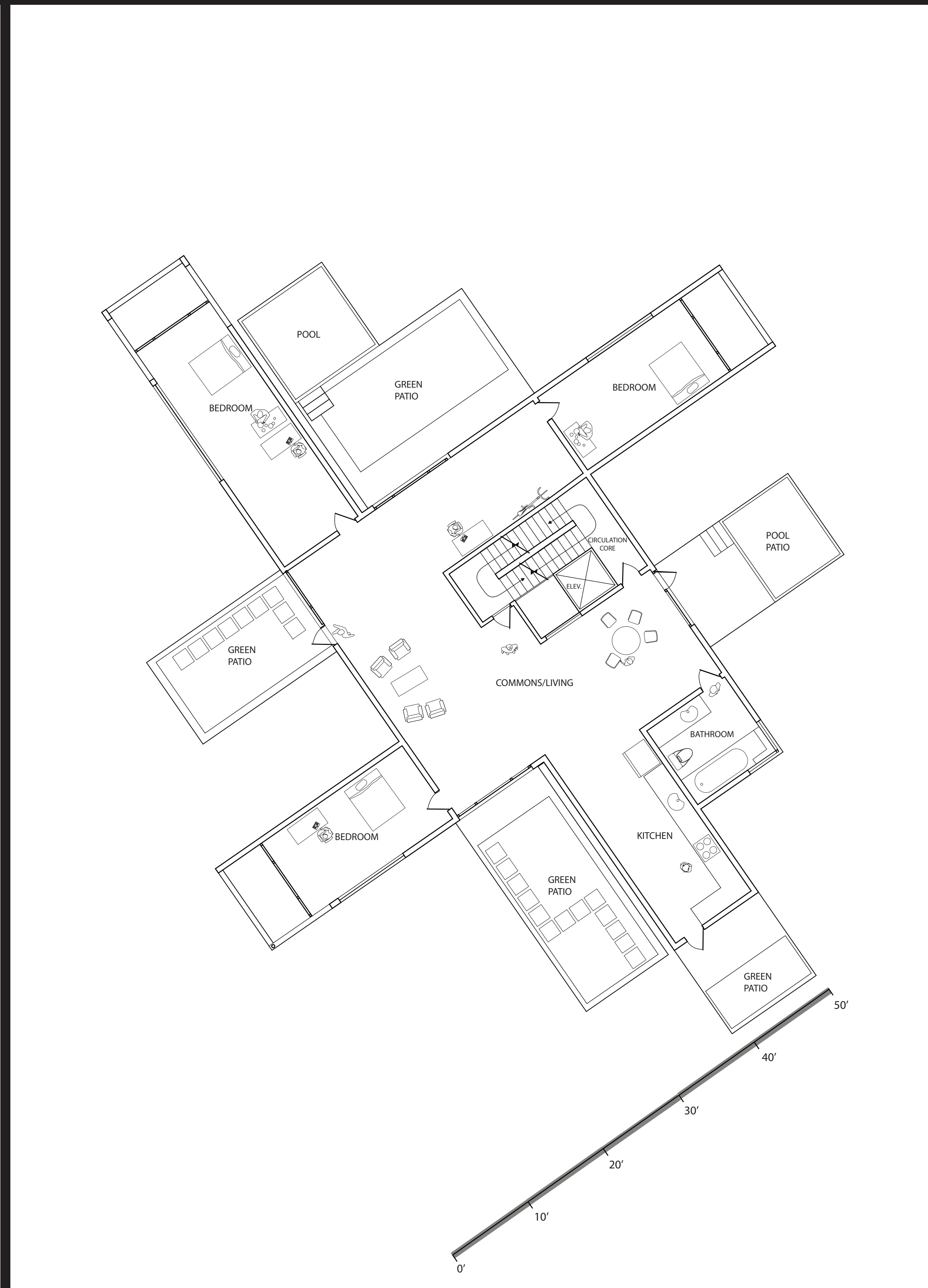
LIVE + WORK COMPLEX - UNIT PLAN
